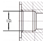
Metric Parallel Female Port
